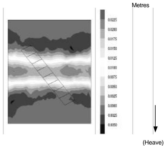
Figure 9: Surface settlements from fully-coupled model
