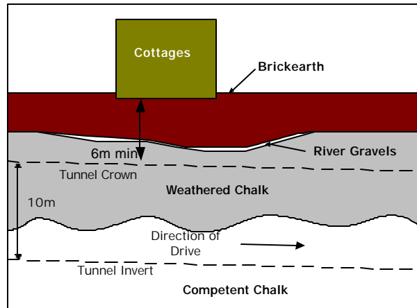
Figure 2: Section through cottages on axis of tunnel
