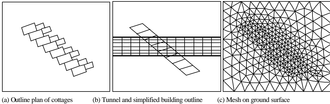
Figure 7: Development stages for the finite element model
