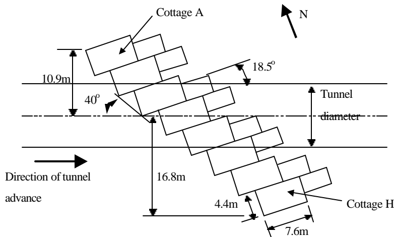
Figure 4: Plan layout on tunnel and cottages
