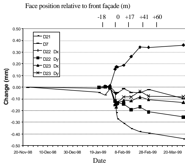
Figure 6: Movement of pre-existing cracks
